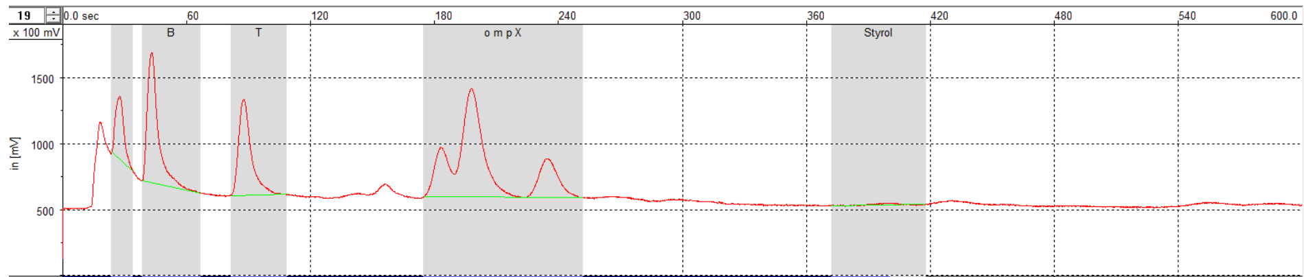
figure 3: 10 ng/l BTX + MTBE with "GC-PID A C"
