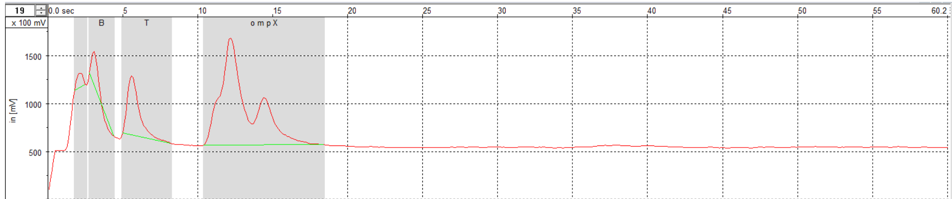
figure 1: 10 ng/l BTX + MTBE with "GC-PID A S"
